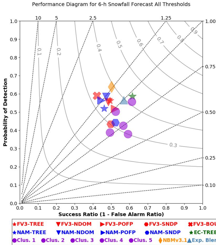
Figure 15. Performance diagram for 6-h forecasts experiment cases of all objects >1", >2", >4" of accumulated snowfall with each marker color denoting the model and each marker type denoting the precipitation type method. Other markers include the 5 clusters (purple circles), NBM v3.1 (orange diamond), and experimental forecast blend (light blue triangle). The dashed lines in the plot indicate bias and the curved lines indicate CSI/Threat Score.
