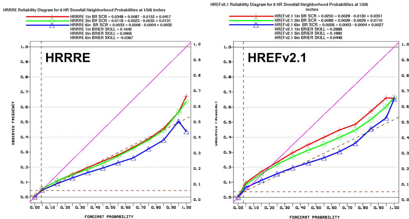
Figure 26. Reliability diagrams for the HRRRE (left) and HREFv2.1 (right). Colors and markers represent the 6-hour neighborhood probability snowfall threshold used as 1 (red), 3 (green) or 6 (blue) inches.
