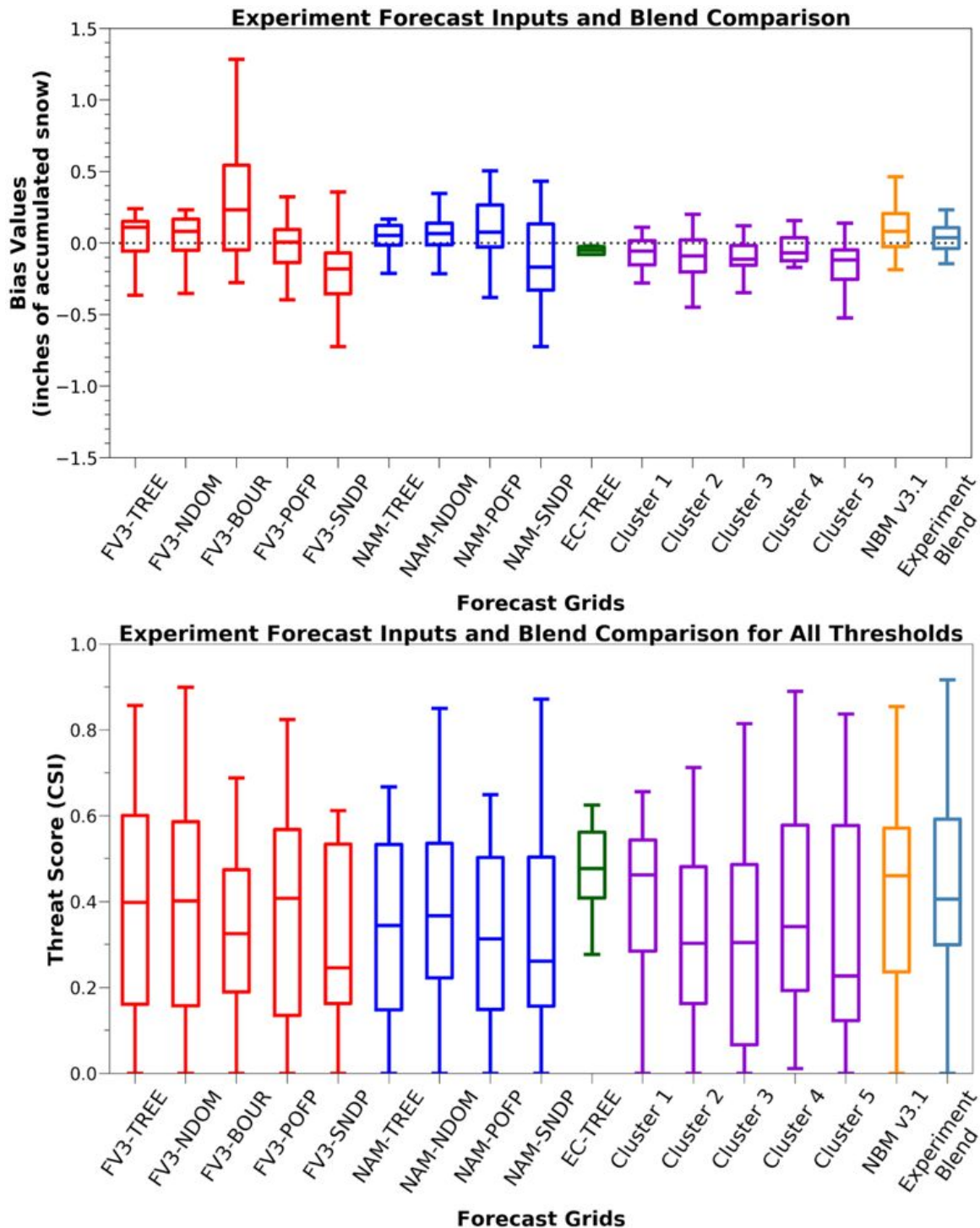
Figure 14. Distribution of bias (top panel) and CSI/Threat score (bottom panel) values for each precipitation type experimental guidance for the FV3 (red), NAM-12 (blue), ECMWF (green), clusters (purple), NBM v3.1 (orange), and experimental forecast blend (light blue). The bar within the rectangle indicates the median of the distribution. The bounds of the box reflect the 75th (top) and 25th (bottom) percentiles of the values. The whiskers extend to the lowest and highest values. A bias of 0 is indicated by the gray dashed line.
