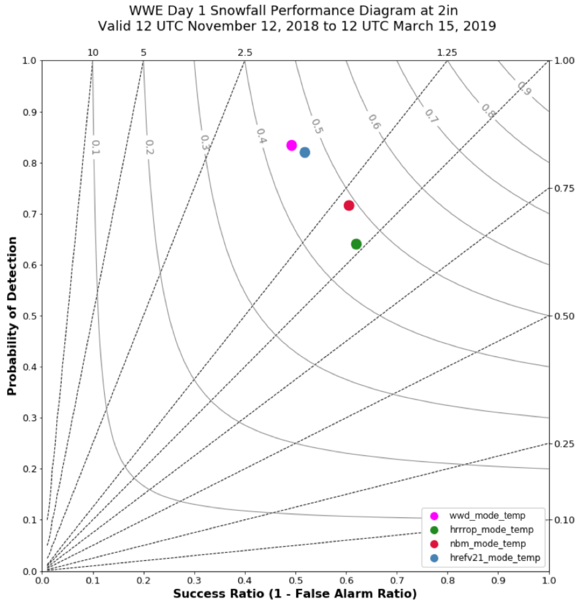
Figure 27. Performance diagram for season-long statistics of 24-h forecasts of objects >2" of accumulated snowfall with each marker color denoting the model used. The dashed lines in the plot indicate bias and the curved lines indicate CSI/Threat Score.
