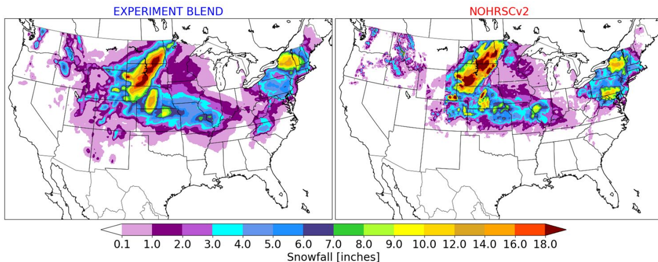
Figure 9. Total aggregated snowfall from all 19 events from the experiment blend (left) and observed NOHRSCv2 amounts (right). The 13-14 March 2019 blizzard is prominent due to the fact that it comprised 4 out of all 19 events.
