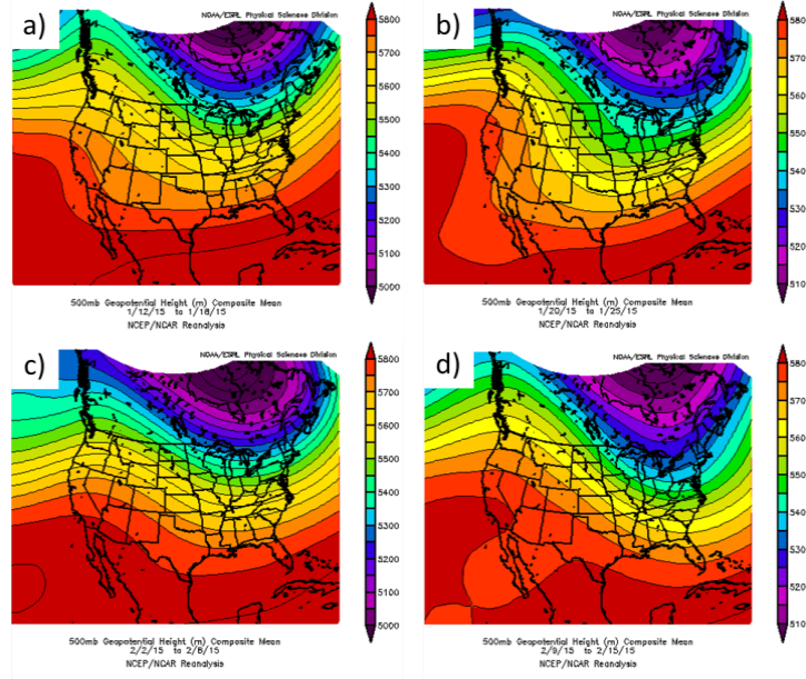
Figure 3. Composite mean 500 hPa heights for the 4 week experiment period: (a) 12-18 Jan, (b) 20-25 Jan, (c) 2-8 Feb, and (d) 9-15 Feb, 2015. Images generated from the NCEP/NCAR Reanalysis provided by NOAA/ESRL/PSD ( http://www.esrl.noaa.gov/psd/data/composites/day/ ).
