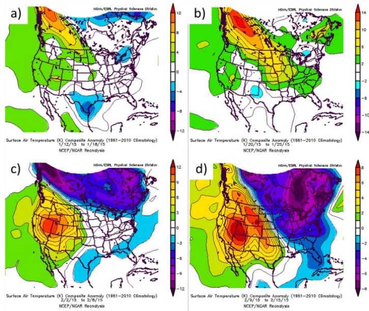
Figure 4. Composite mean surface temperature (K) anomalies for the 4 week experiment period: (a) 12-18 Jan, (b) 20-25 Jan, (c) 2-8 Feb, and (d) 9-15 Feb, 2015. Images generated from the NCEP/NCAR Reanalysis provided by NOAA/ESRL/PSD ( http://www.esrl.noaa.gov/psd/data/composites/day/ ).
